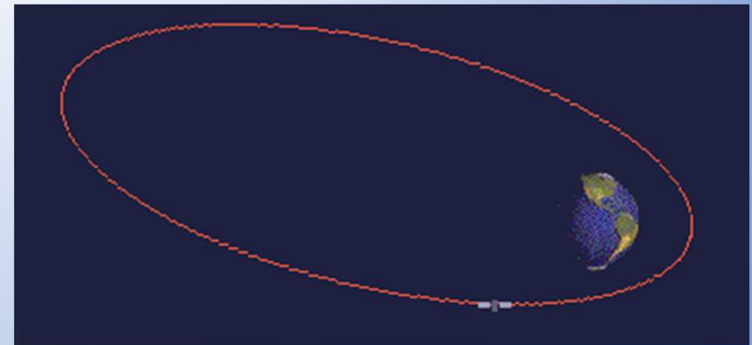
Elliptical Orbit
